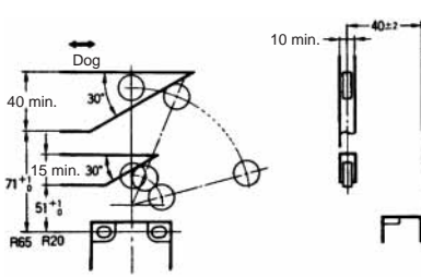
Roller Plunger (D4D-□□32R)
